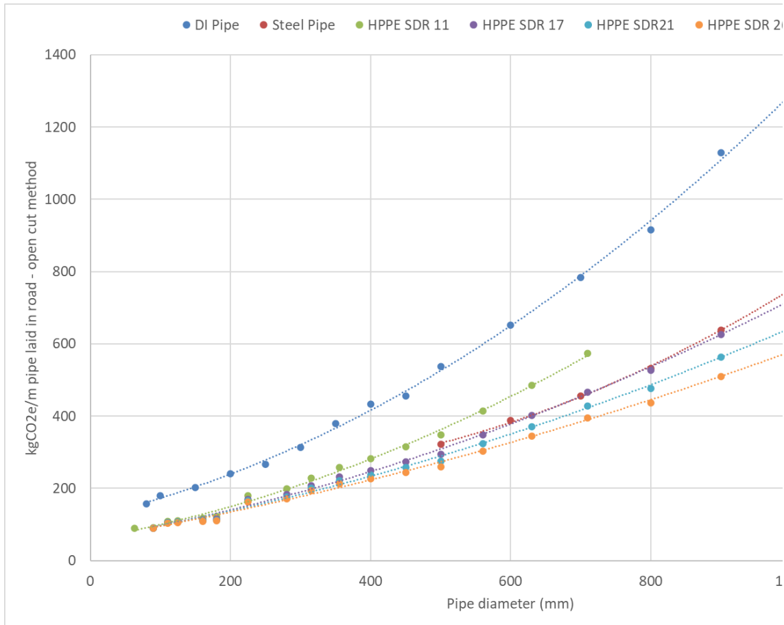
Figure 7.3: Overview of estimated embodied carbon impact of different pipe materials
