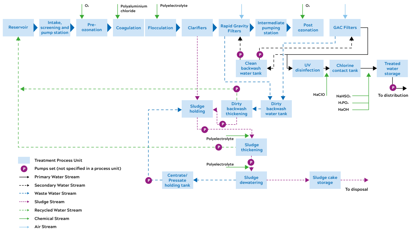
Figure 6: The indicative treatment process for SLR
