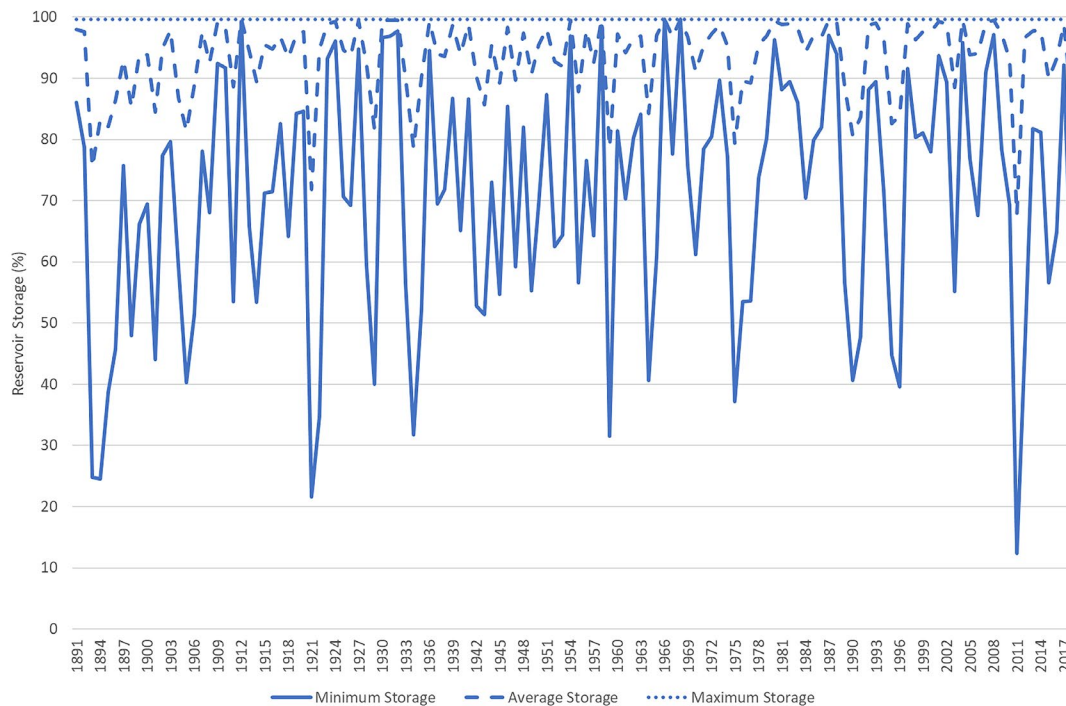
Figure 10: South Lincs Reservoir storage during a historical + mid-climate change simulation
