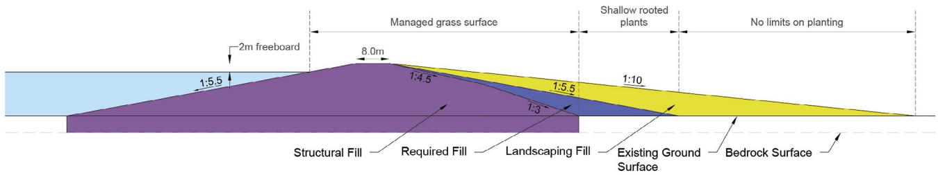
Figure 5: Typical embankment cross section
